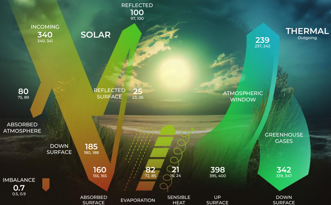
Figure 6: Global mean energy budget of the Earth according to the IPCC (values expressed in W/m^2 , uncertainty ranges shown in parentheses). 22
